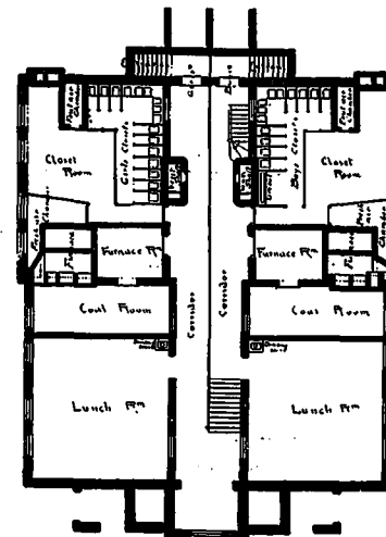
Basement Plan
