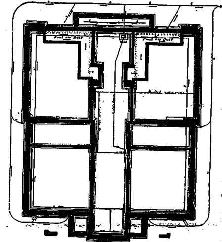
Foundation
