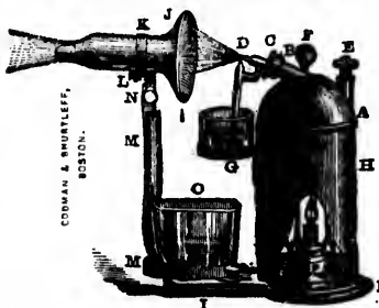
The Complete Steam Atomizer, No. 15 (Pat.).
