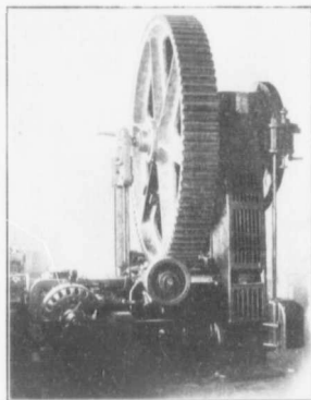
90" diam., 12" face, 5700 lbs., 88 teeth, 1 diam. pitch.
