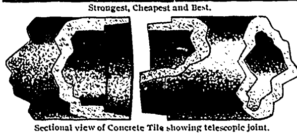
Sectional view of Concrete Tile showing telescopic joint.
