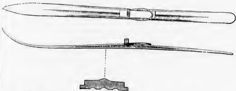
THE "SKI" OF THE EXPEDITION IN PLAN, ELEVATION, AND SECTION.
