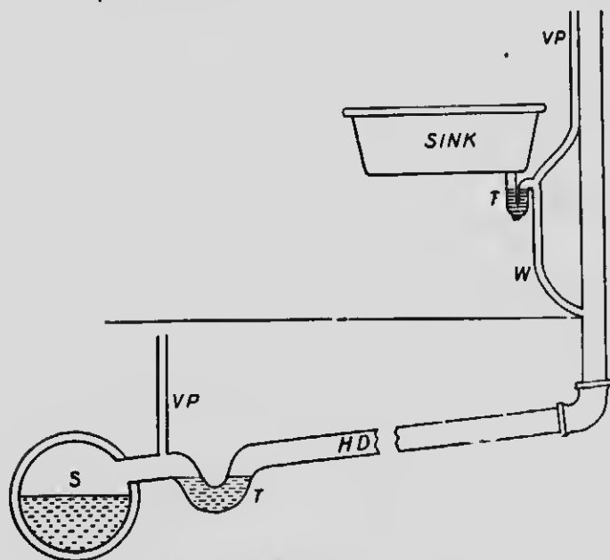
Sink and sewer connection
