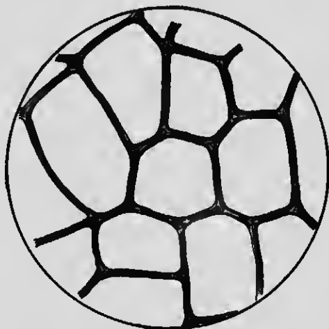
Cellular structure of a potato
