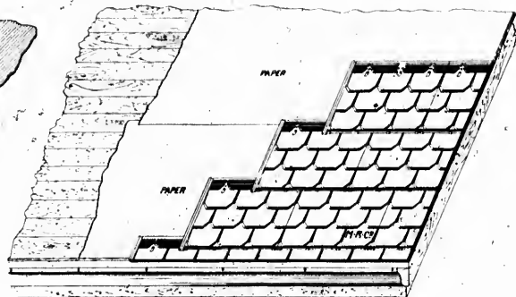
Fig. 11. "Eastlake" Shingles as applied to a roof.
