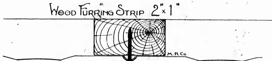
Fig. 3403.—Section of Joint on Plates Nos. 417, 488, and 489.
