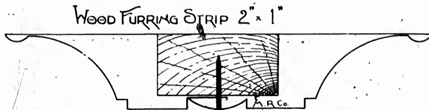
Fig. 3400.—Section of Joint on Plates Nos. 400, 401, 402, 403, and 479.
