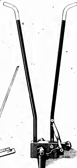
Fig. 5. Combination Squeezing and Punching Tool. Patented 1900.
