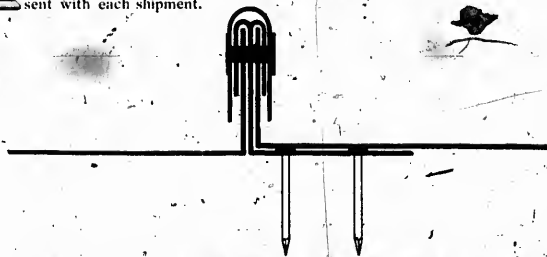
Fig. 44.—Shows Standing Seam complete with Cleat, and Rivetted.
