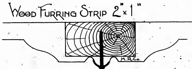
Fig. 3401.—Section of Joint on Plates Nos. 405, 406, 407, 408, 409, 410, 411, 415 and 478.
