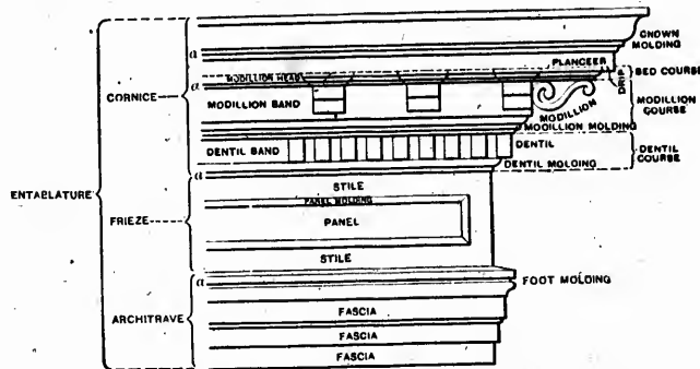
Fig. 220—The Several Parts of a Cornice.
