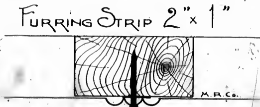
Fig. 3407. Section of Joint on Plates Nos. 416 and 422.
