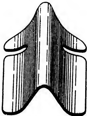
Fig. 142.—Lead plate for nasal arch.
