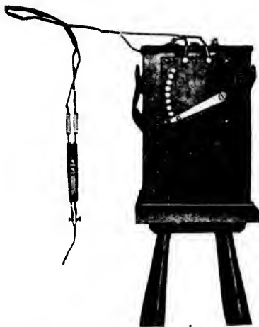
Fig. 47.—Ballard galvanocautery-battery, with cord, handle, and knife.
