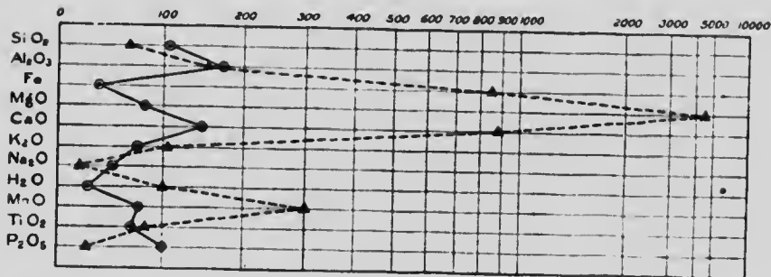
Figure 1. Diagram illustrating hornblendization and aplitization. The hornblendite alteration is indicated by the solid line, the aplite alteration by the broken line.
