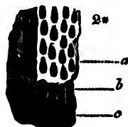
Stictopora ramosa , natural size and enlarged.†
