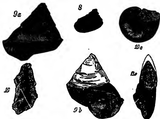
8, 9a, 9b, 10c, 13e, Pleurolomaria — of Trenton limestone. 16, Murchisonia gracilis do
