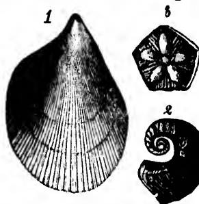
1, Ambonychia radinta . 2, Joint of the Glyptocrinus decadactylus , a crinoidean fossil very common. 3, Cyrtolites ornatus .
