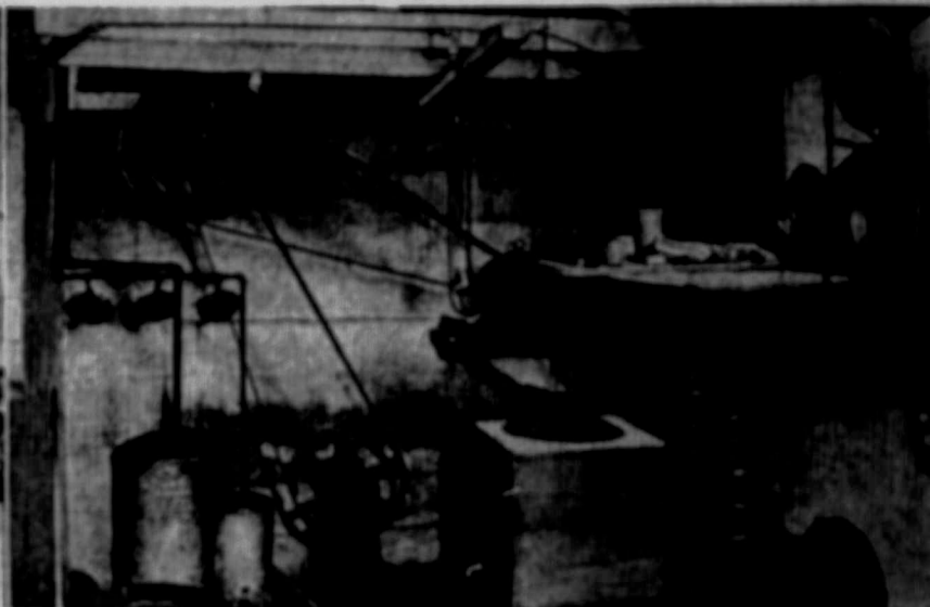
Hydro Power in the Dairy turns the Separator, operates the Milking Machine, or heats water for washing utensils.
