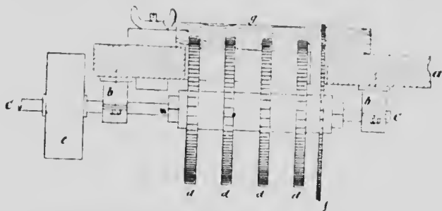
Fig. 51.—Apparatus for growing and cutting Pencil Boards
