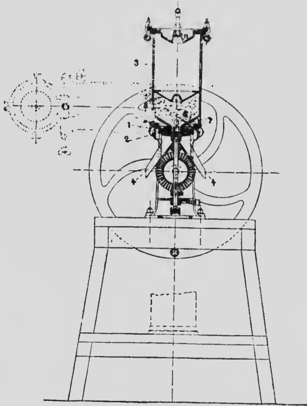
Fig. 44.—Talmie's Graphite Mill.
