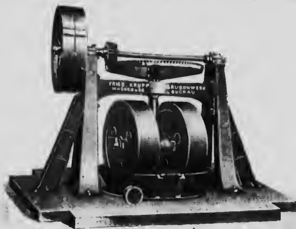
Fig. 27.—Edgestone Mill.
