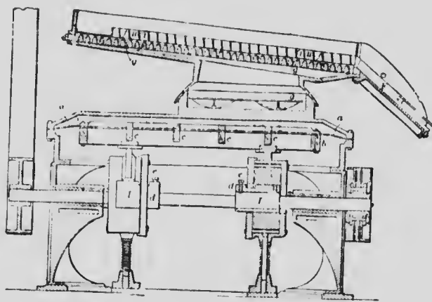
Fig. 25. Longitudinal Section. Scale \frac{1}{4} inch = 1 foot.
