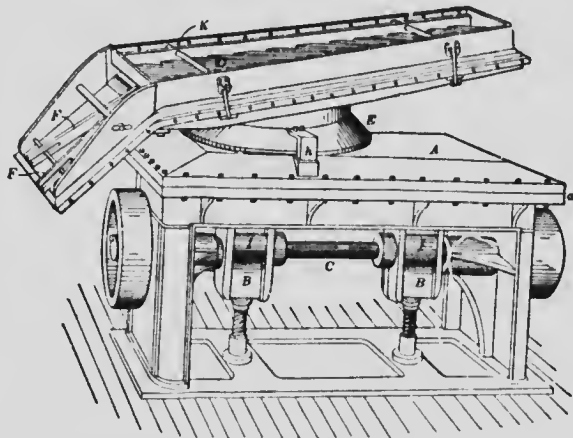
Fig. 24.- Perspective of the Hooper Pneumatic Concentrator.]
