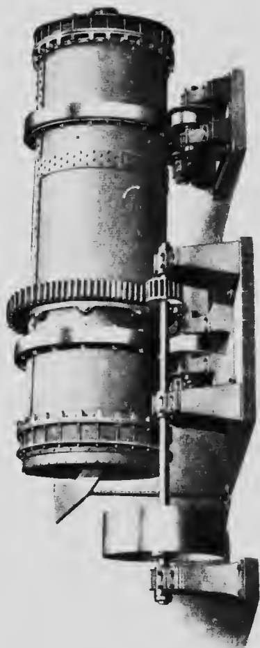
Pebble Tube Mill as Constructed by the Abbe Engineering Co., of New York.
