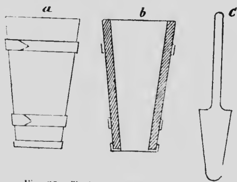
Fig. 35.—Tools for making Crucibles.
