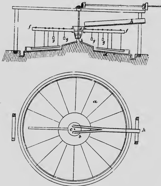
Fig. 30.—Circular Buddle.
