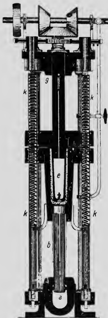
Fig. 36.—Apparatus for the manufacture of Crucibles.
