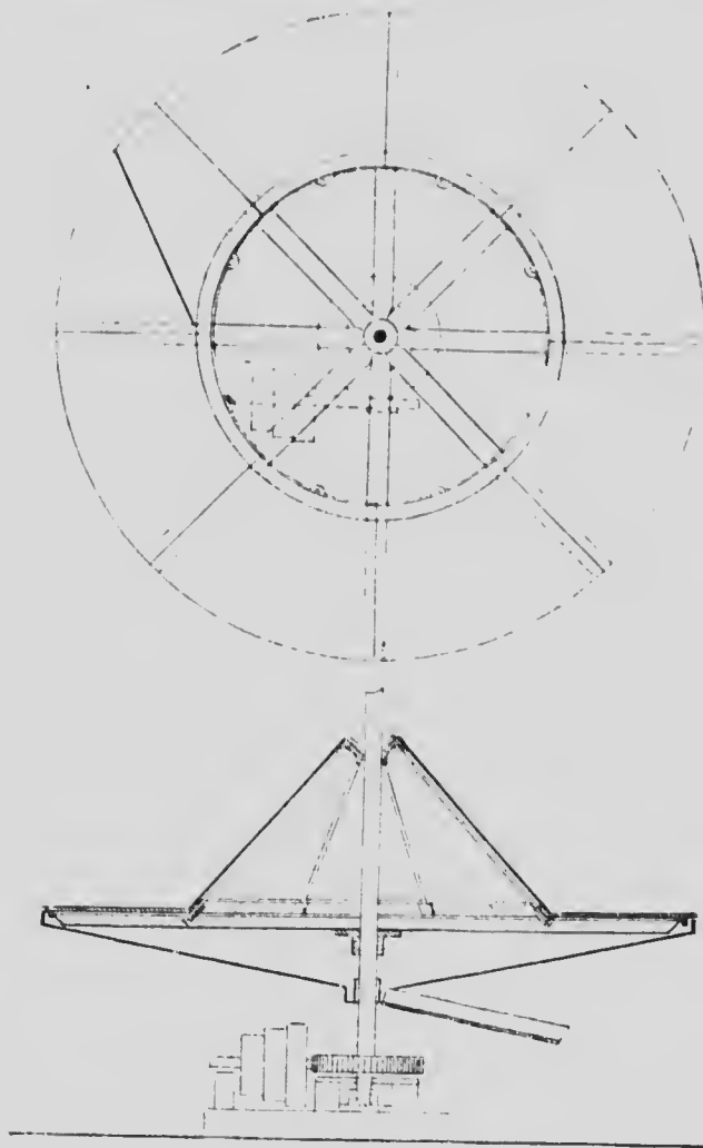
Fig. 17.—Revolving Ore-picking Table
