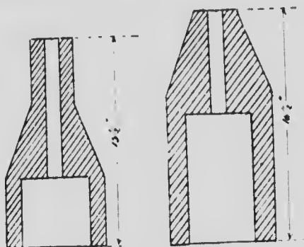
Fig. 41.—Phosphorizers.
