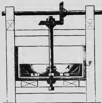
Fig. 43.—Conte's Graphite Mill.
