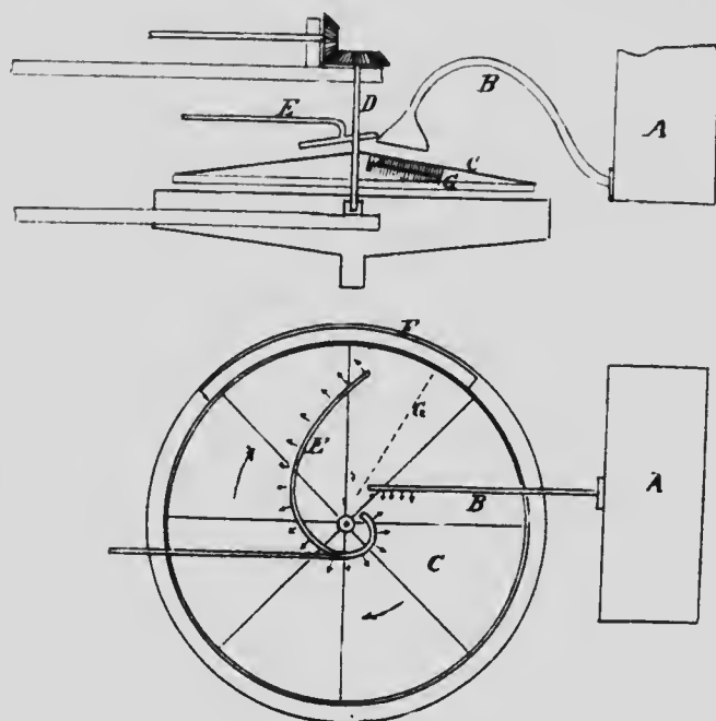
Fig. 31.—Horizontal Revolving Sizing Sieve.
