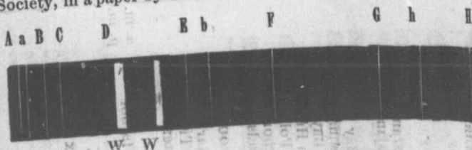
Position of the auroral bands compared with the principal lines of the Solar spectrum.—A to H, from Fraunhofer's lines; C, E, G, h, hydrogen; D, sodium; b, magnesium; W, W, bands in aurora and zodiacal light.
