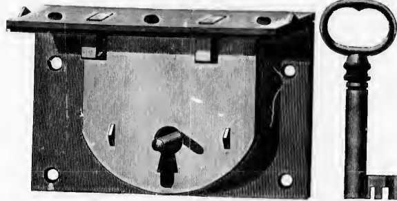
Full Size Cut of No. 5.
