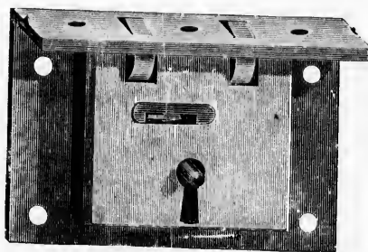
Full Size Cut of No. 205, 2 1/2 Inch.
