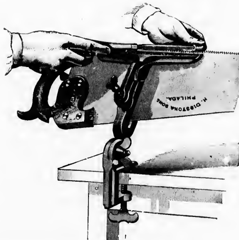
No. 2, Disston's Adjustable Saw Clamp,
