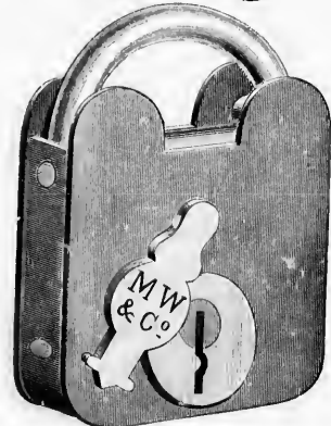
Full Size Cut of No. 1029.
