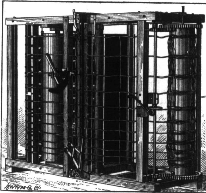
THE AMERICAN WIRE FENCE MACHINE.
