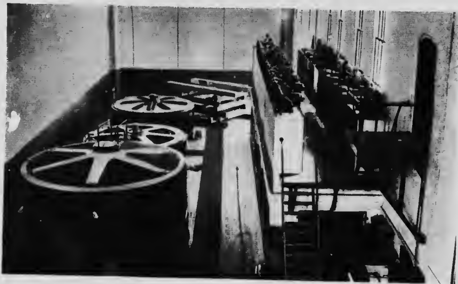
Kootenay River Development. Generator Room, No. 2 Plant, Upper Bonnington Falls.
