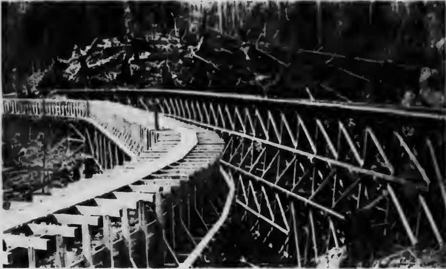
Vancouver Island Power Company Limited. Flume and Railroad on trestle.
