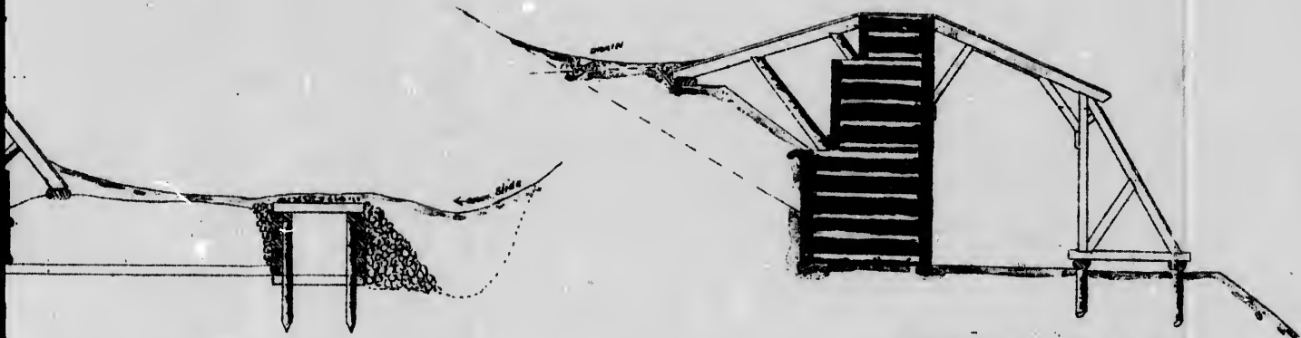
TYPICAL SHED.
