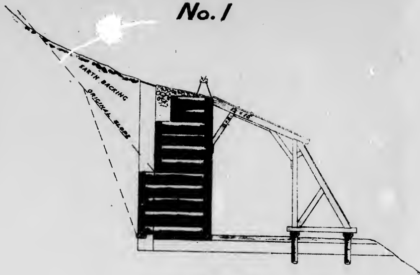
TYPICAL SHED.
