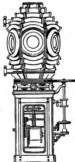
HOLOPHOTAL REVOLVING LIGHT. (FOURTH ORDER.)
