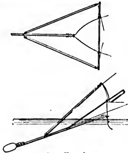
Spar Torpedo. (Front and side views.)
