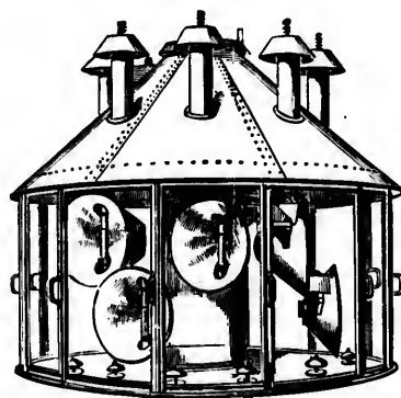
FLOATING LIGHT LANTERN.
