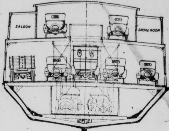
Sectional view of the "Motor Princess" showing method of storing cars.
