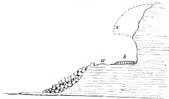
Fig: 2.—REMAINS OF CAVERN ON PASS OF NAHR-EL-KELB.
