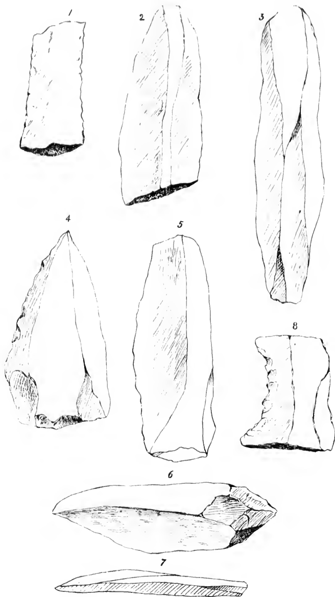
1. Fragment of Spear, Ras, Beyroul. 2, Knife, Do. 3, Knife, Ant Elias. 4, 5, Knives, Nahr-el-Kelb. 6, 7, Knife and Spicule, Helouan. 8. Modern Strike-light, worn on one side.
