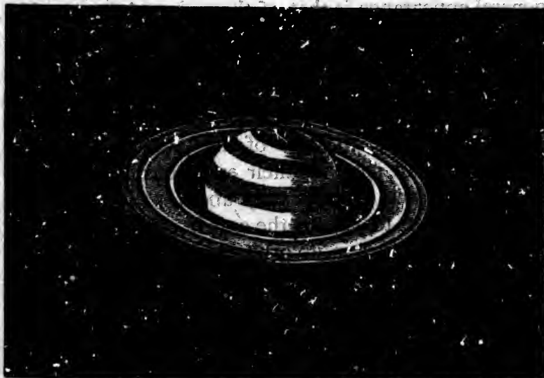
FIG. 36.—Saturn and his rings.
