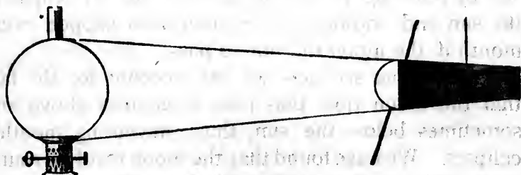
FIG. 25.—Eclipse of the Moon.
