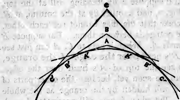
FIG. 4.—Diagram explaining how it is that the higher we go the further we can see. To an eye at A the edge is at A'A' , to an eye at B the edge is at B'B' , and so on.
