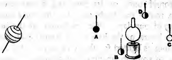
FIG. 28. — Diagram illustrating the motions and appearances of a body between us and the sun.
