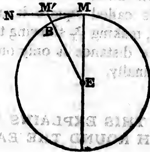
FIG. 48.—The fall of the Moon towards the Earth.
