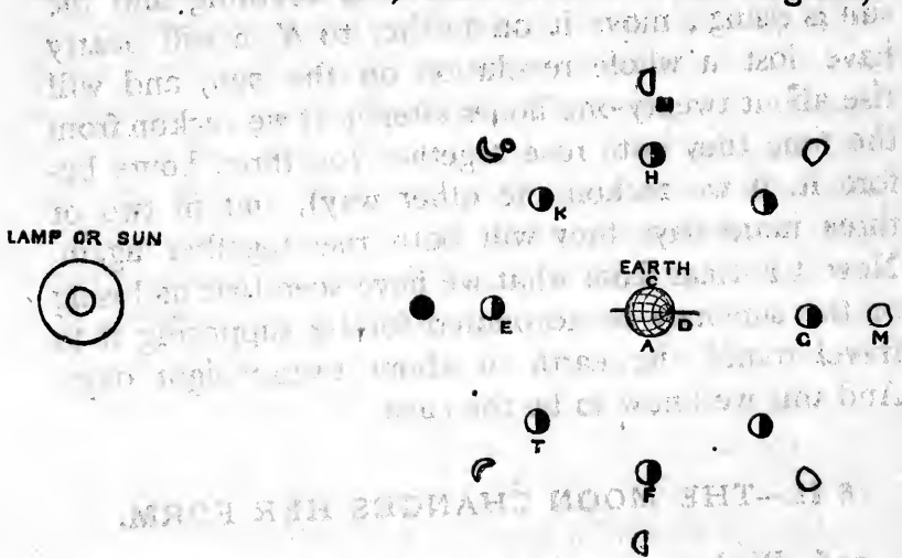
FIG. 22.—The Moon's motion round the Earth.
