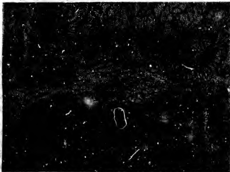
FIG. 40.—A Sun-spot.
