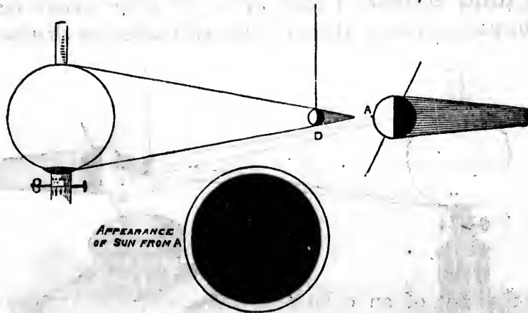
FIG. 24.—Annular Eclipse of the Sun.
