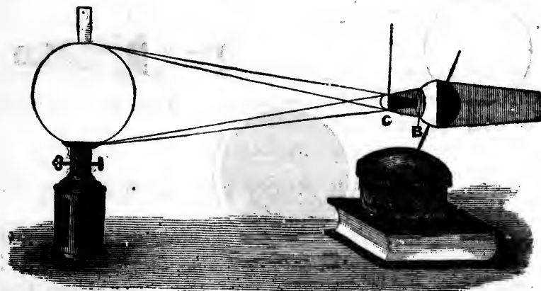
FIG. 23.—Total Eclipse of the Sun.
