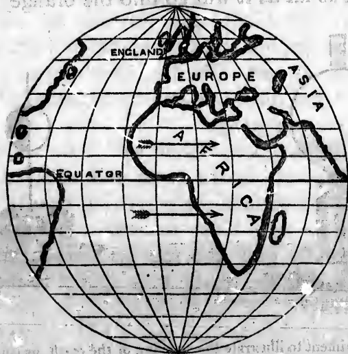
FIG. 9.—The direction of the earth's spin.
