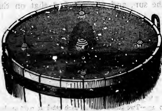
Fig. 12.—The plane of the Ecliptic.
