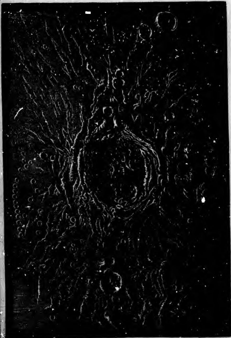
A Lunar Crater.
