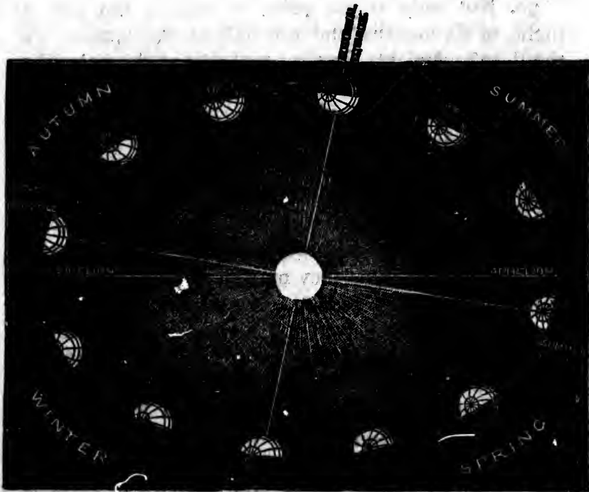
FIG. 20.—Explanation of the Seasons.
