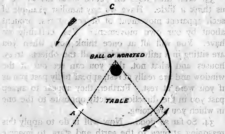
Fig. 7.—Diagram explaining Fig. 6; with the direction of motion indicated a body at A is setting, at B is rising, and at C is overhead.
