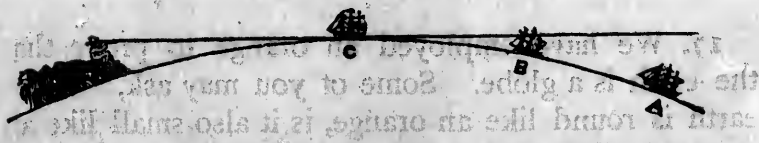
FIG. 3.—Diagram showing how, when we suppose the earth is round, we explain how it is that ships at sea appear as they do. At A the ship is invisible, at B its topmasts begin to be seen, and at C it is in full sight.
