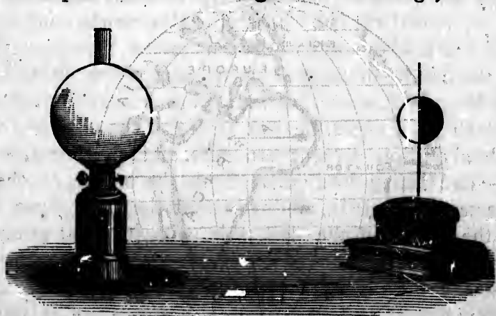
FIG. 10.—Experiment to illustrate the spinning of the earth, as causing day and night.
