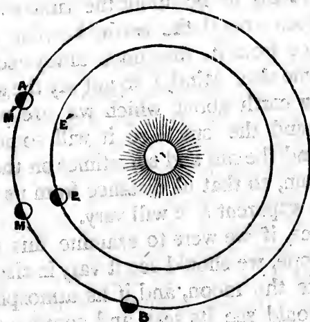
FIG. 29.—Diagram illustrating the motion of a body travelling round the sun outside the orbit of the earth.
