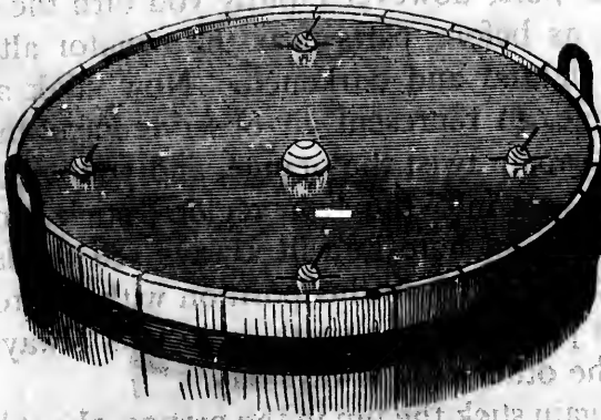
FIG. 15.—Earth with inclined axis of rotation.
