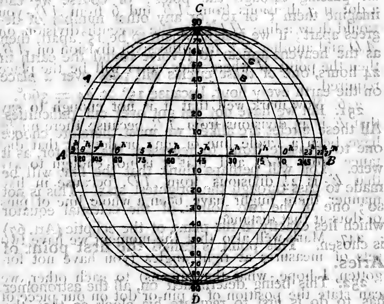
FIG. 47.—How the positions of stars are stated.
