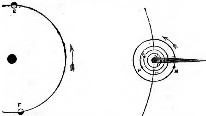
FIG. 35. — Diagram explaining the eclipses, occultations, and transits of Jupiter's satellites.
