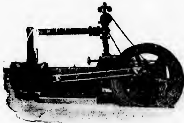
Straight-Line Steam-Driven Compressor.
