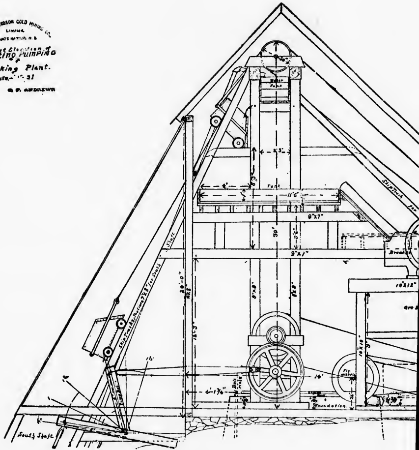
Richardson Gold Mining Company—Hoisting, P
