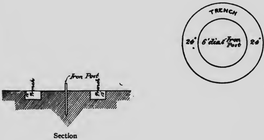
Witness Iron Post and Trench Fig. 7
