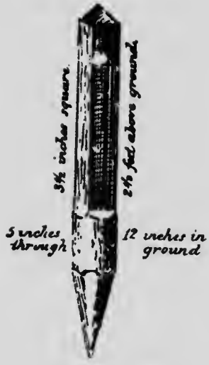
Wooden Post Fig. 2
