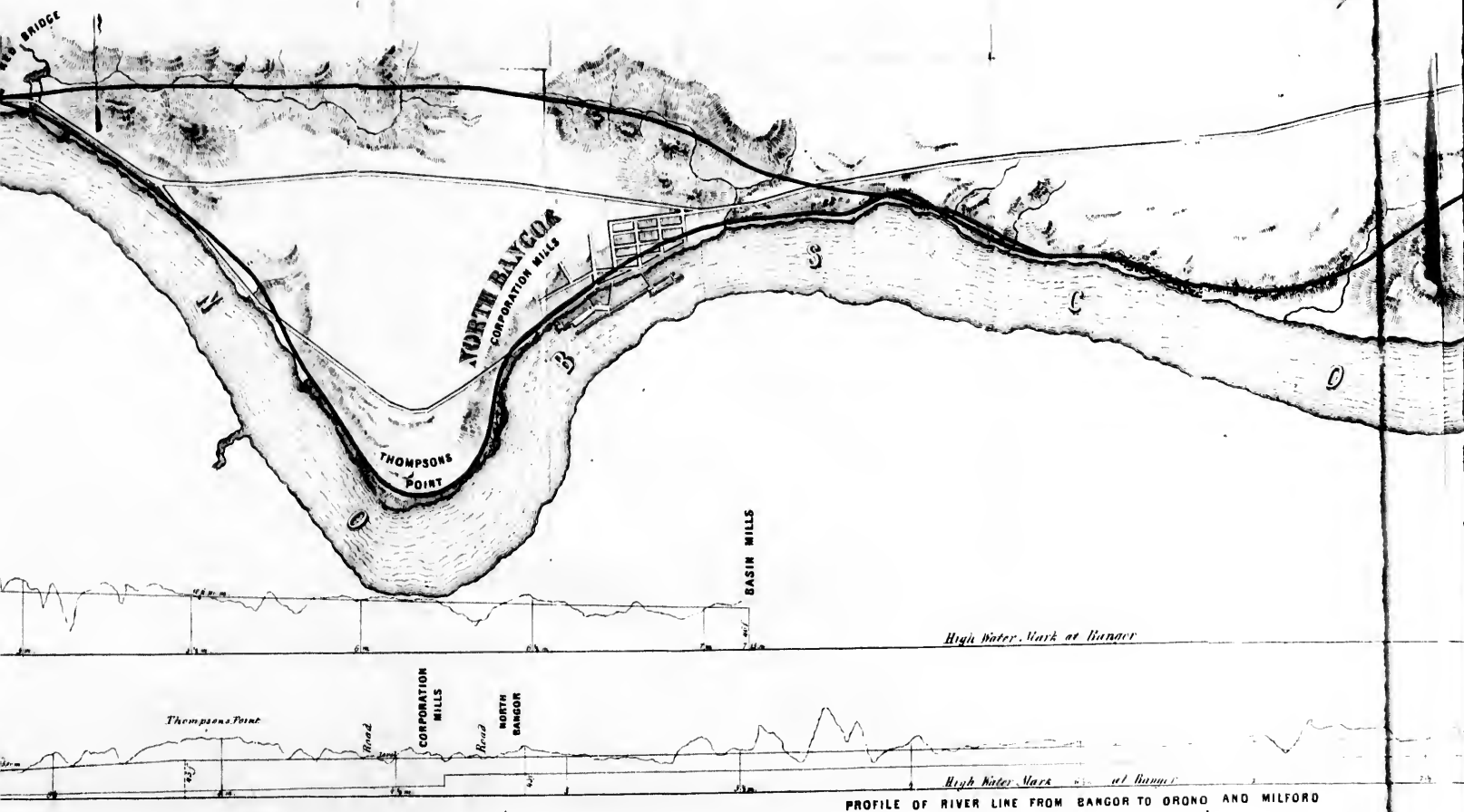
PROFILE OF RIVER LINE FROM BANGOR TO ORONO AND MILFORD
