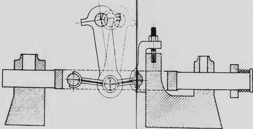
— Longitudinal Section on C.D. —
