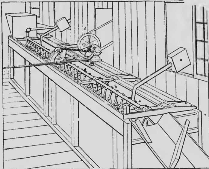
Fig 7. Sectional elevation and perspective of Scaife trough washer.
