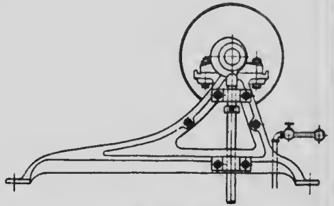
— Cam Driven Jig. — End Elevation.
