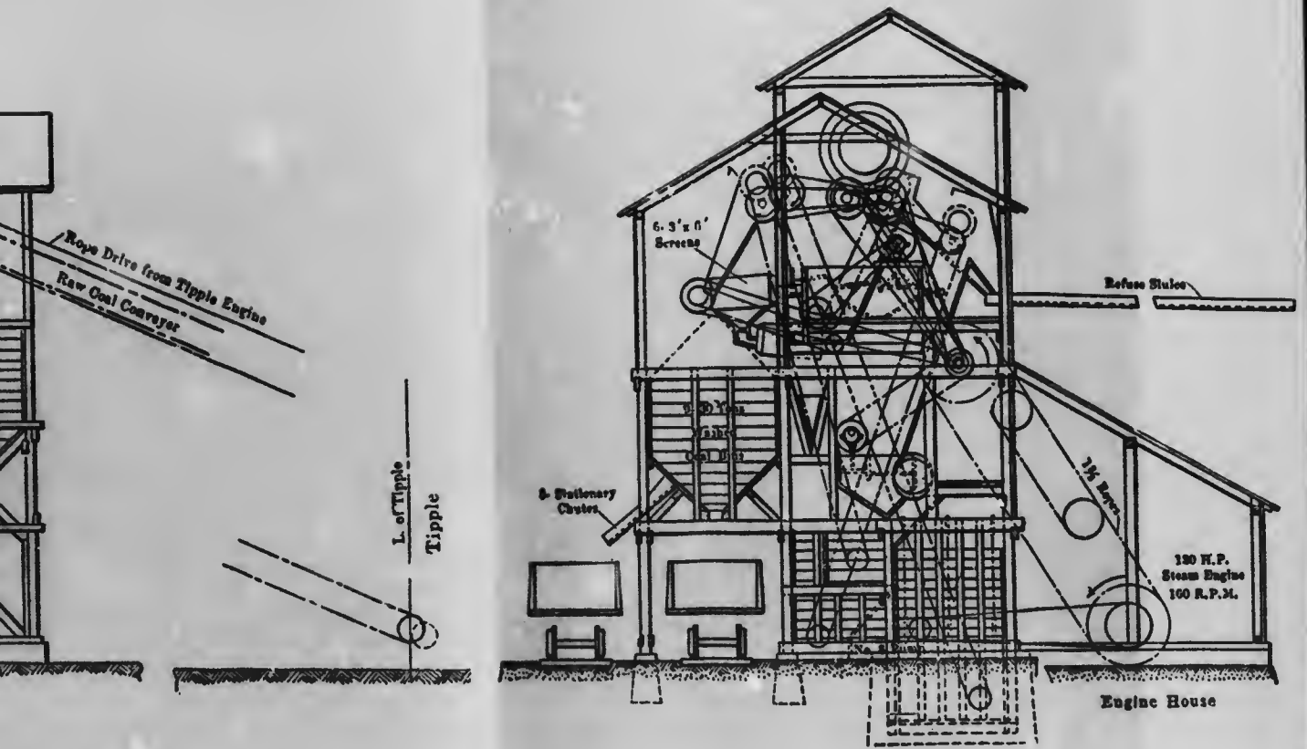
Side and end elevations of a Luhrig washery.
