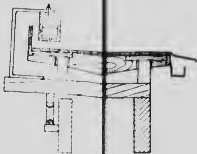
— Cross Section on A.B. —
