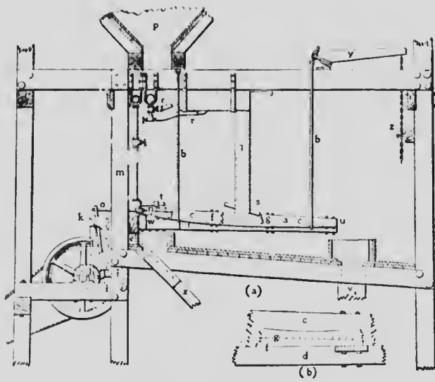
Fig.17. The Campbell table.
