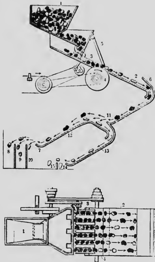
Fig. 26. Elevation and plan of Langerfield dry separator (slate picker).
