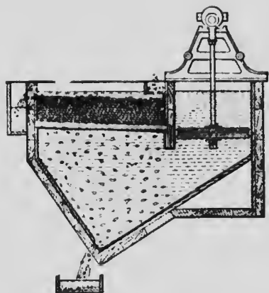
Fig. 12 (a). Vertical section Luhrig nut-coal jig.
