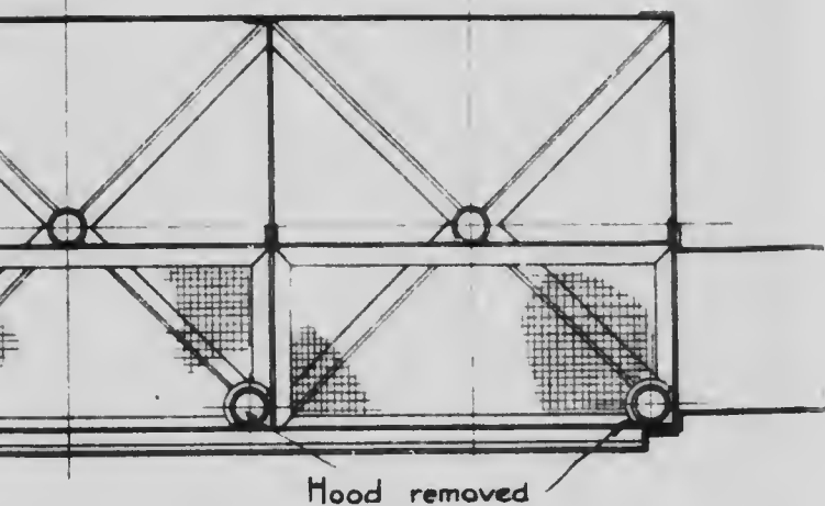
— Plan of Jig Box. —
