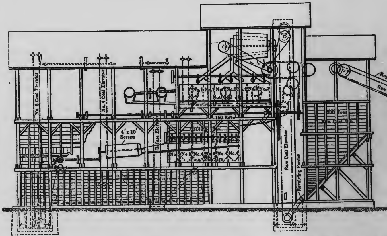
Fig. 21. Side and end elevations.
