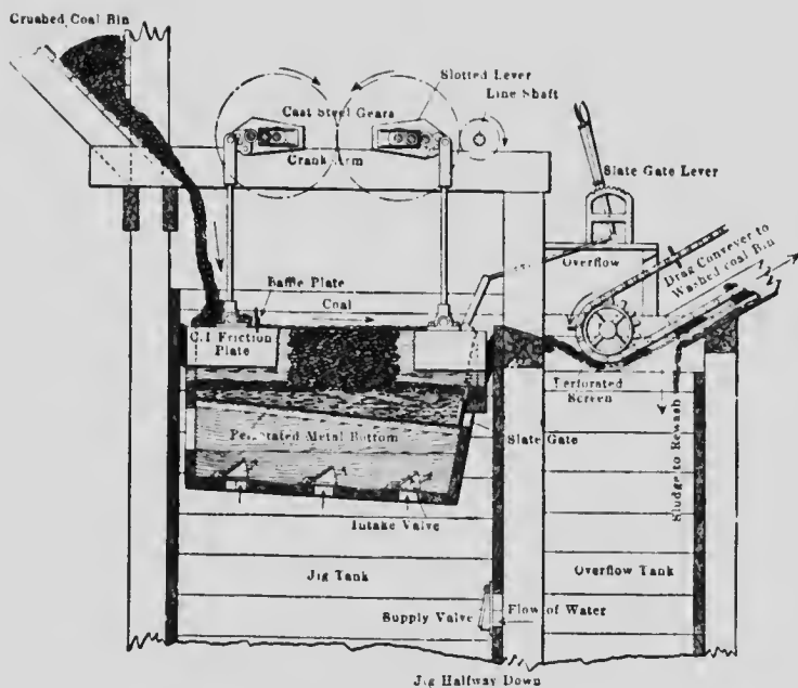
Fig. 16. Pittsburgh movable sieve coal jig.
