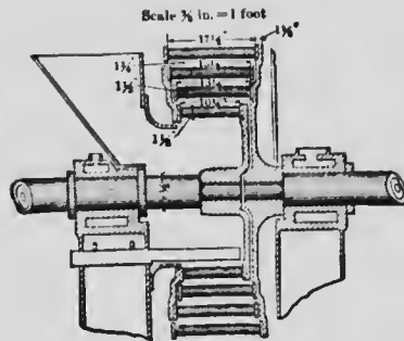
Fig. 4 (a). Sectional elevation of Stedman (Carr) disintegrator.
