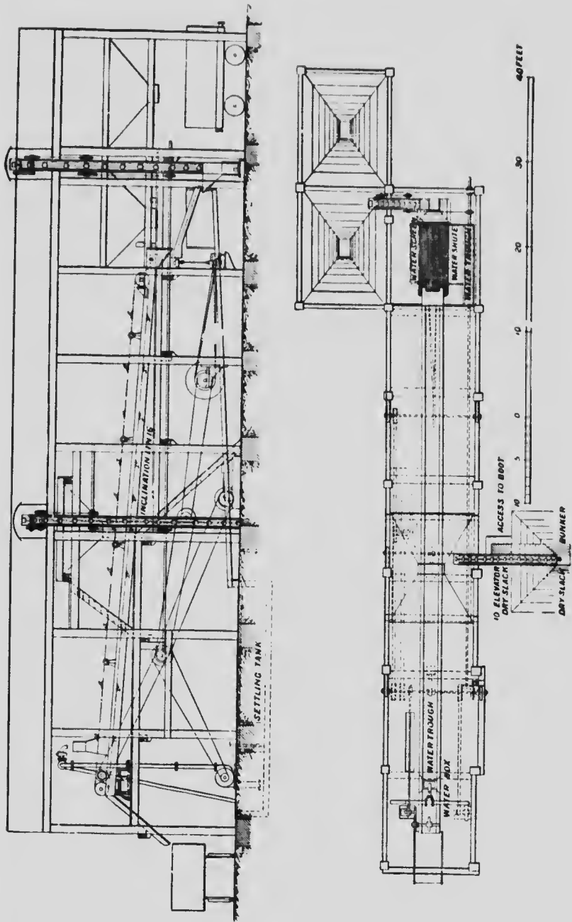
Fig. 8. Elevation and plan of Elliott washer.
