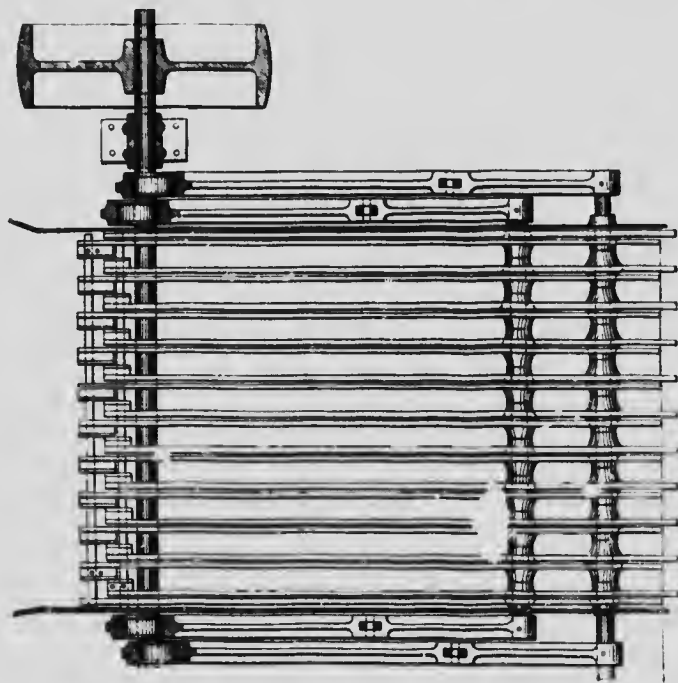
Fig. 5. Elevation and plan of Coxé movable bar screen.
