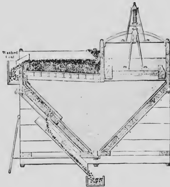
Fig. 14. Vertical section New Century nut-coal jig
