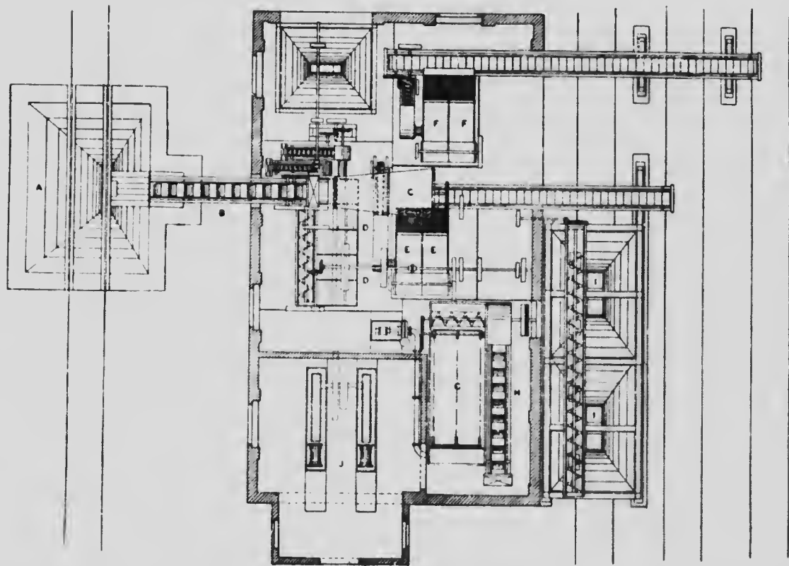
Fig. 19 Elevation and plan of a 350-ton capacity Sheppard washery.
