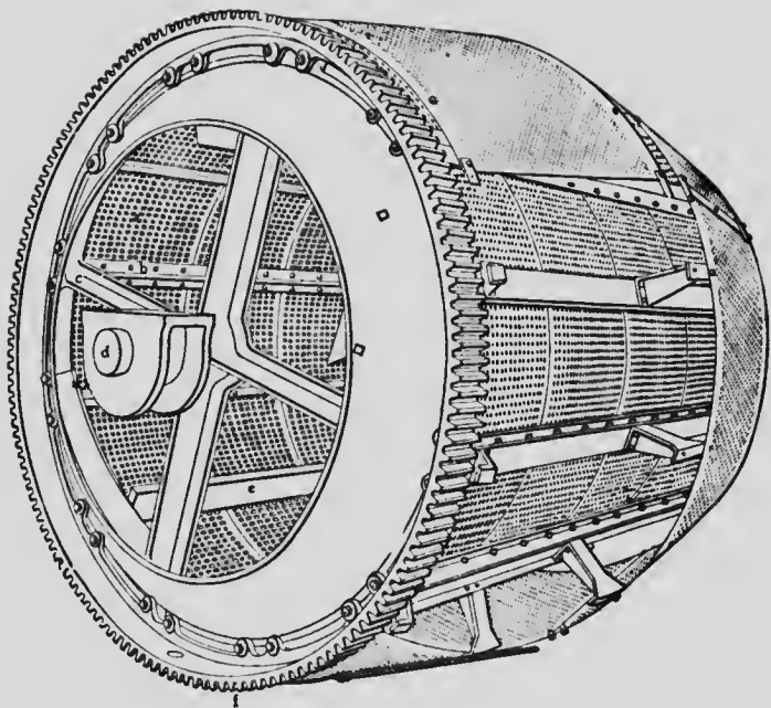
Fig. 2 Bradford coal breaker.
