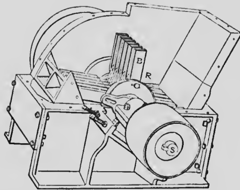
Fig. 3 (a). Swing-hammer pulverizer without cover
