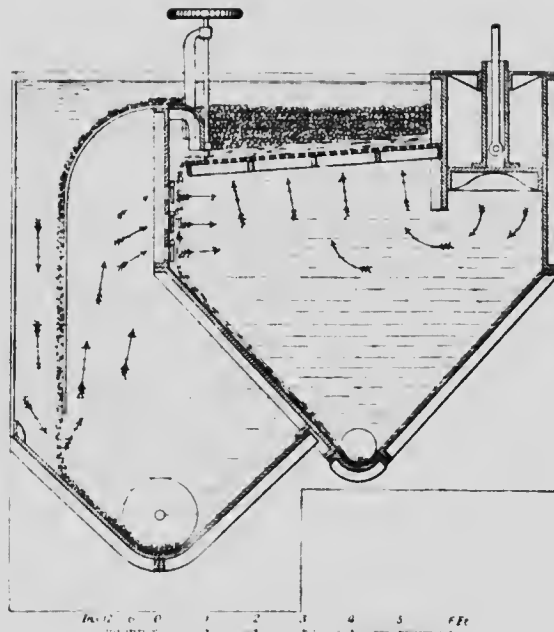
Fig. 15 Vertical section Sheppard nut-coal jig.
