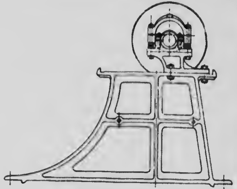
— Eccentric Driven Jig. — End Elevation.
