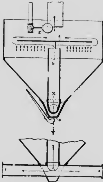
Fig. 24. Sectional elevations of Ramsey sludge tank.
