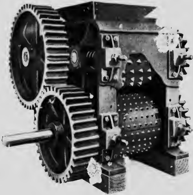
Figure 1. Four roll coal crusher.
