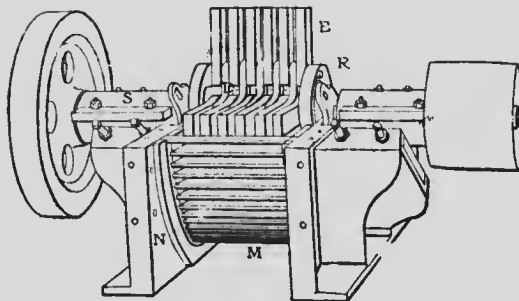
Fig. 3 (b). Swing-hammer pulverizer with housing completely removed.
