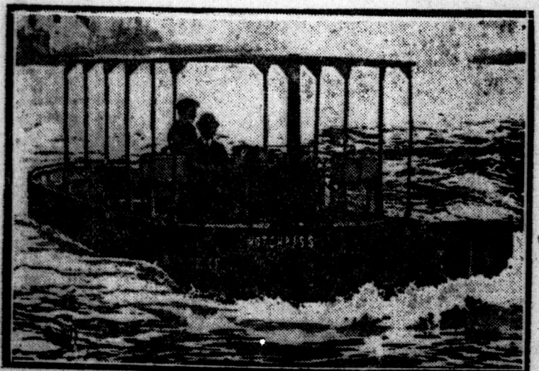
A tug barge driven by internal propellers on a hydraulic principle is seen on the Thames river, England. The draught is reduced to eleven inches and the propeller can also be used as a bilge pump.
