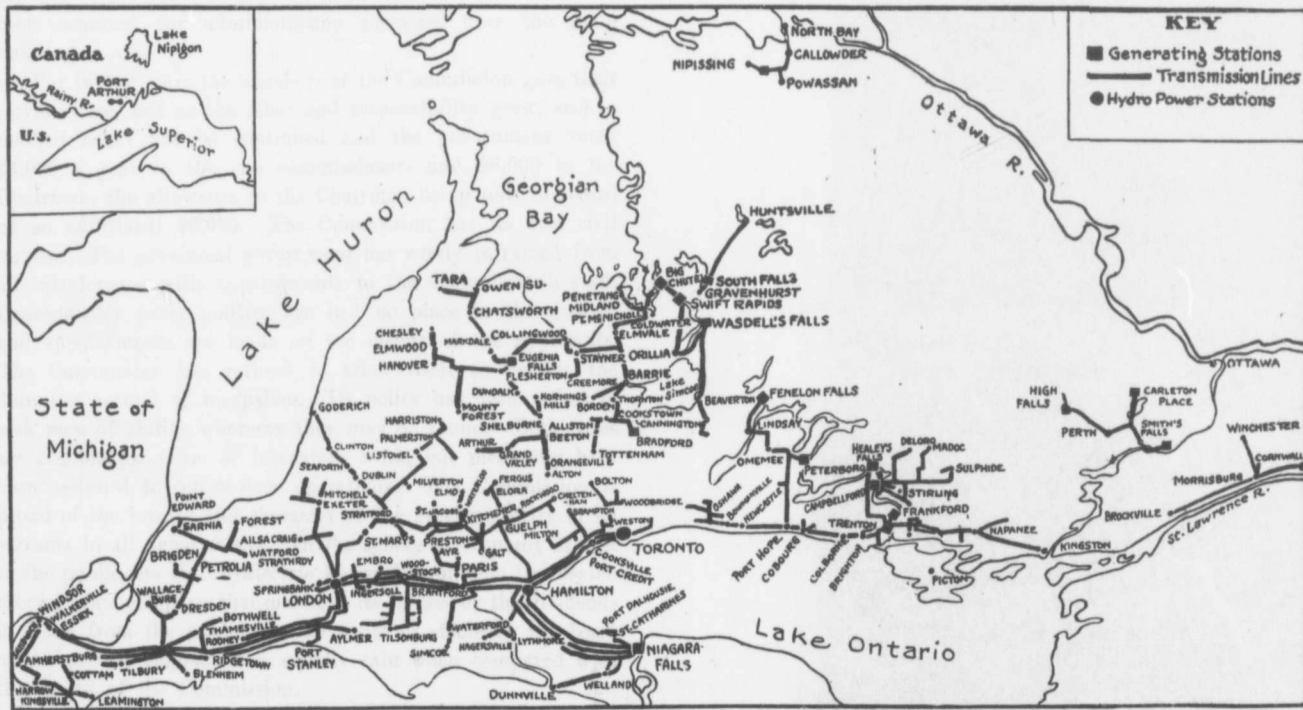
Transmission Lines of the Hydro-Electric Power Commission of Ontario at October 31, 1919.
