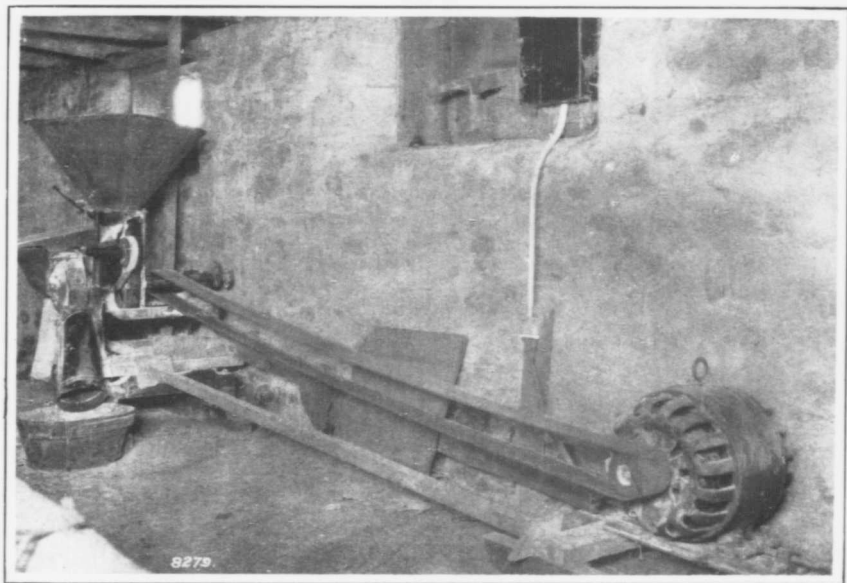
A Feed Cutter Operated by Hydro Power.
