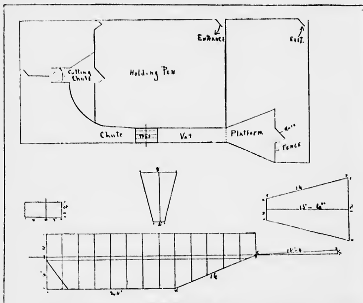
FIG. 170.—Diagram of sheep pen, showing location of dipping vat below.
