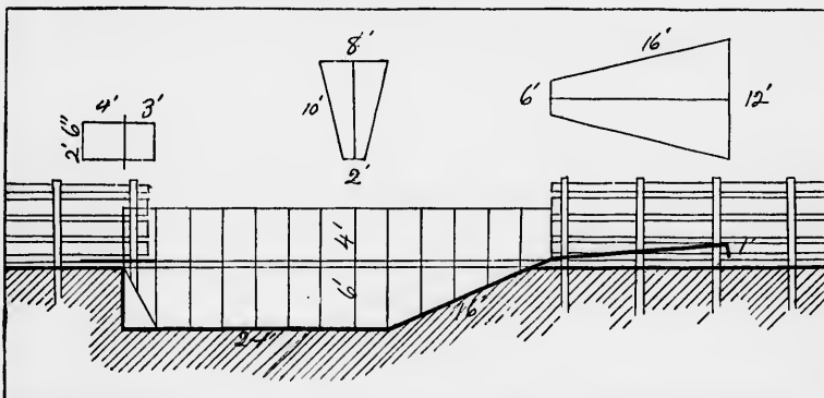
FIG. 169.—Section of dipping vat.
