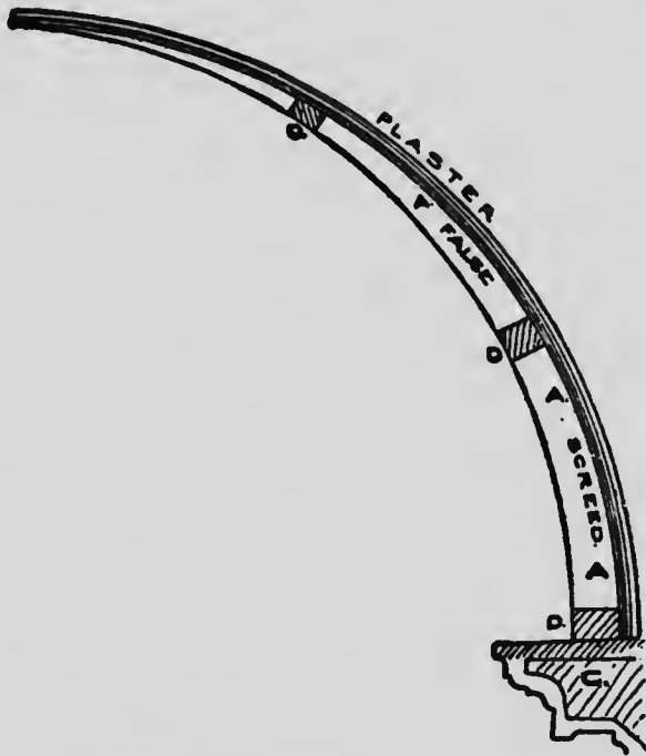
SECTION DOUBLE DIMINISHED MOULDINGS— FALSE SCREED METHOD.
