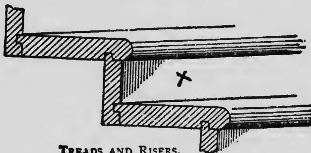
TREADS AND RISERS. NO. 25.
