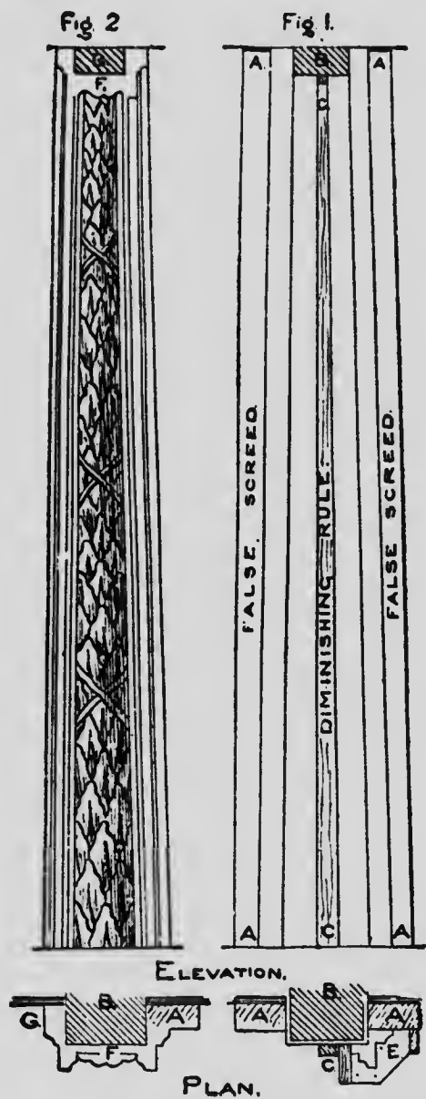
ELEVATION DOUBLE DIMI- NISHED MOULDINGS—FALSE SCREED, METHOD.
