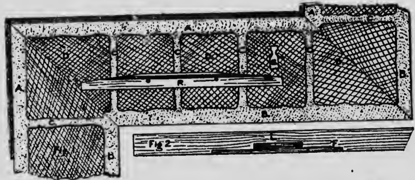
-FIG. 1. FLOATING COVES. FIG. 2. LEVELLING RULE.
