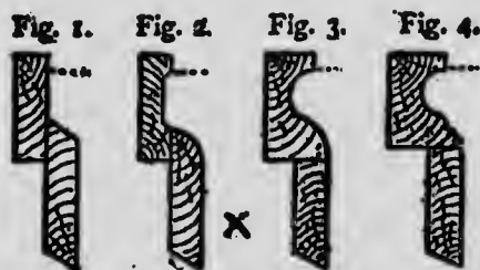
SECTIONS OF NOSING MOULDS WITH RISER BOARDS.
