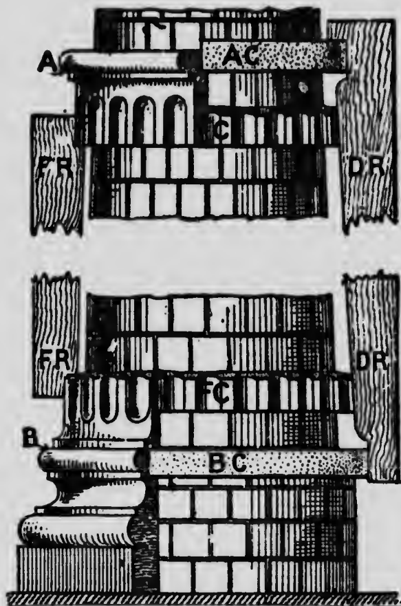
FORMING FLUTED COLUMNS—COLLAR METHOD.
