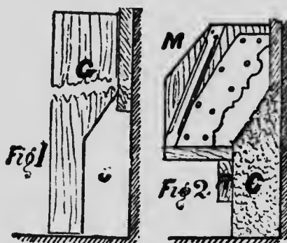
-SKIRTING FORMATION.
