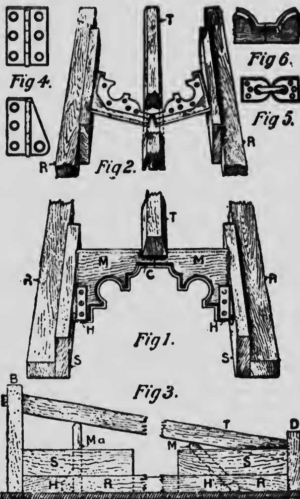
ELEVATIONS, PLAN, AND SECTIONS OF RUNNING MOULD AND RULES FOR DIMINISHED MOULDINGS—TOP-RULE METHOD.
