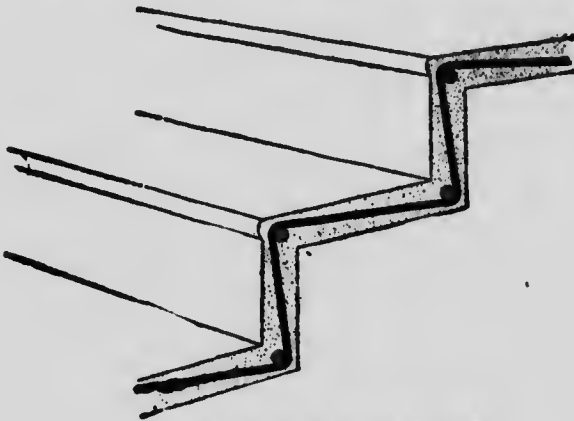
Reinforced concrete steps. NO. 11.
