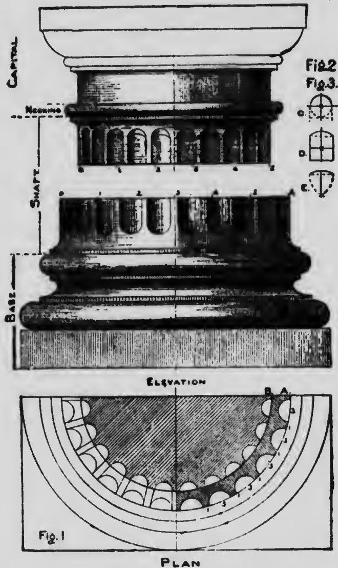
-DIMINISHED FLUTED COLUMNS.
