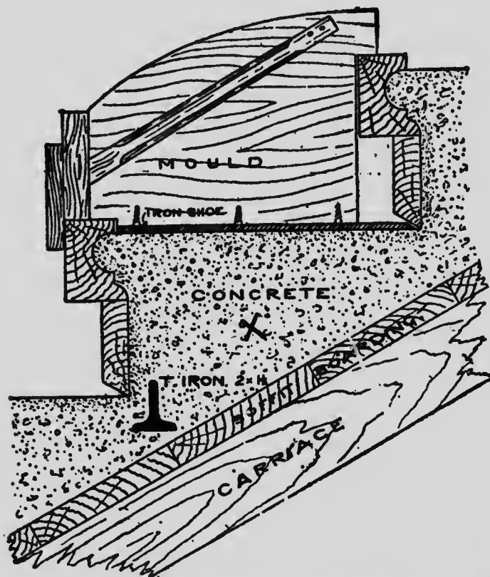
—SECTIONS OF FRAMING OF SOFFIT OF STAIR, RISE AND NOSER MOULD, WITH CONCRETE AND TREAD RUNNING MOULD IN POSITION.
