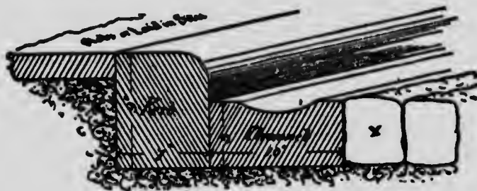
SECTIONS OF CONCRETE CURB, CHANNEL, AND PAVING.
