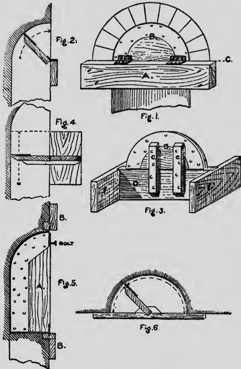
FORMING NICHES WITH RUNNING MOULDS. NO. 23.
