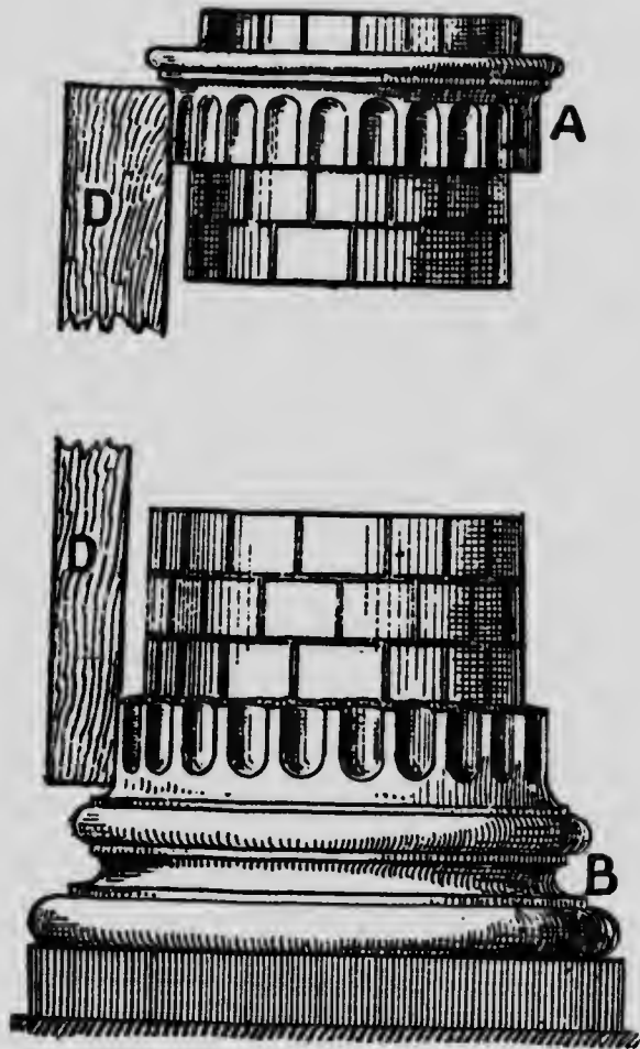
-FLOATED FLUTED COLUMNS, RIM METHOD.
