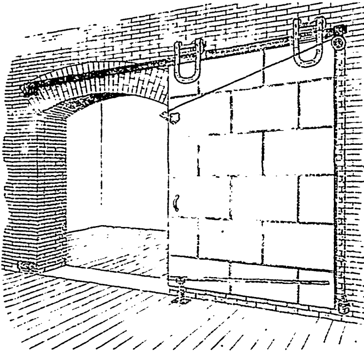
"ACME" AUTOMATIC FIRE DOOR FITTINGS, SET No. 99
