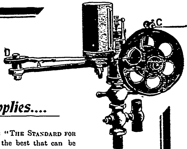
The Improved Thompson Engine Indicator with Reducing motion.
