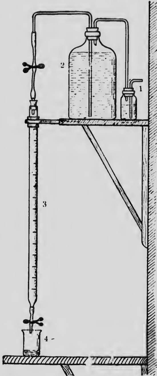
ACIDIMETER.
