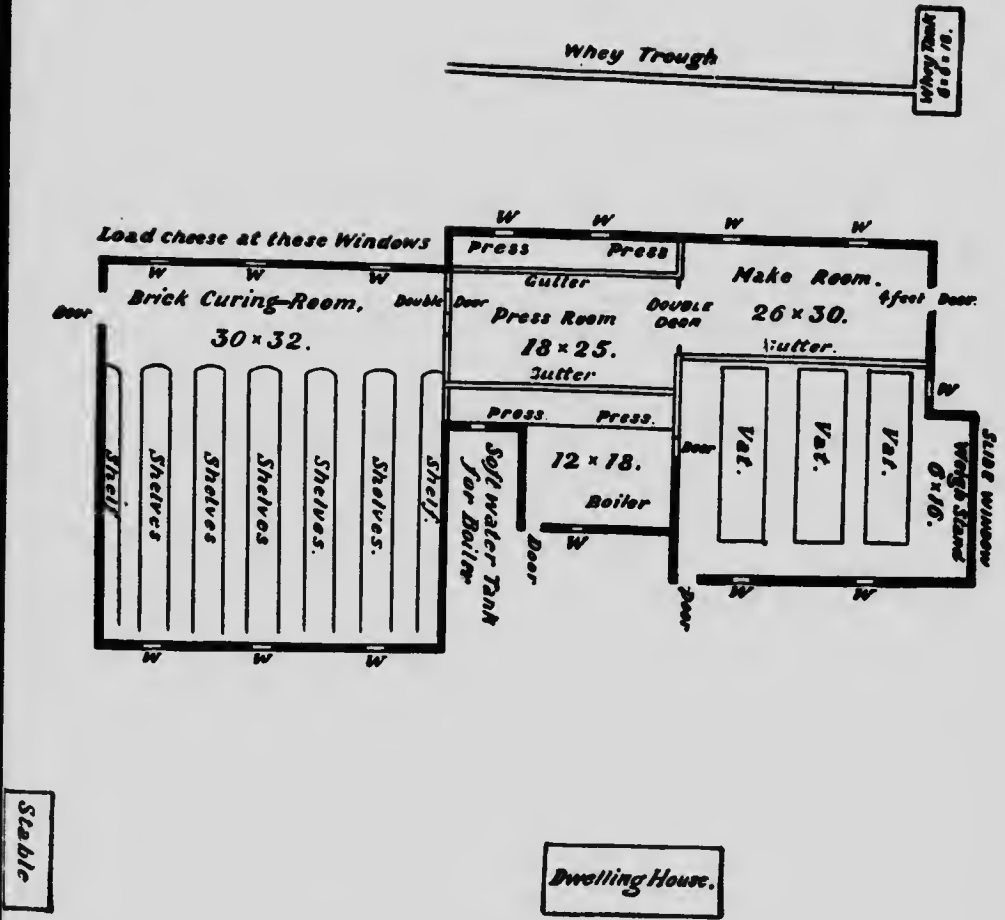
GROUND FLOOR PLAN CHEESERY.
