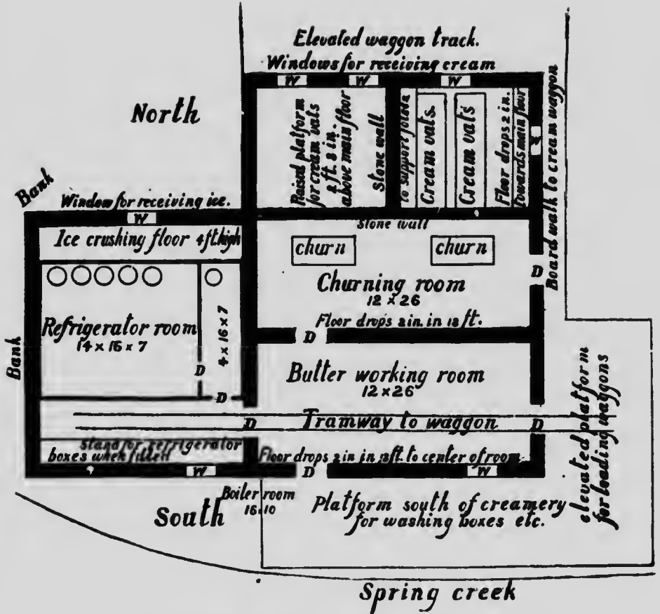
PLAN FOR CREAM-GATHERING CREAMERY.
