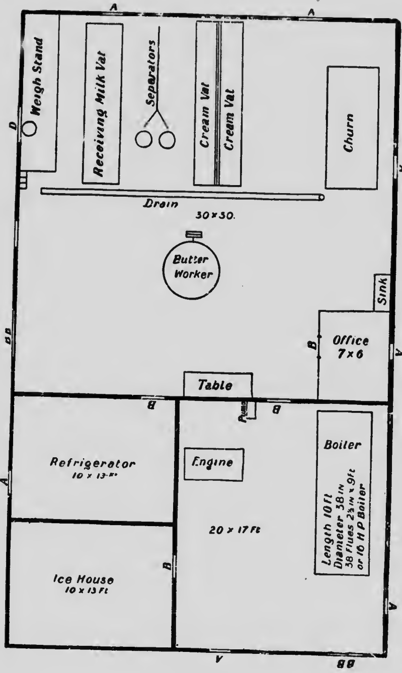
PLAN FOR WHOLE MILK CREAMERY.
