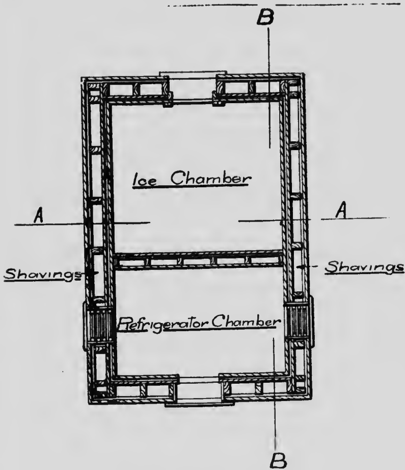
GROUND FLOOR PLAN COMBINED ICE-HOUSE AND REFRIGERATOR.
