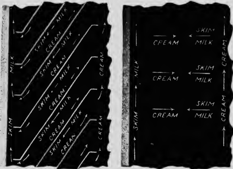
DISC TYPE, SHOWING AVOIDANCE OF CONFLICT BETWEEN CREAM AND SKIM-MILK.
