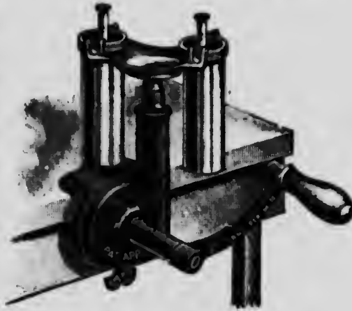
2 BOTTLE HAND BABCOCK TESTER FOR FARM USE.
