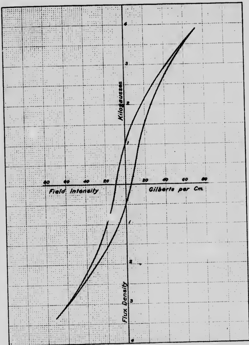
Fig. 5. Hysteresis Loop for Pure Cobalt - Sample H 217
