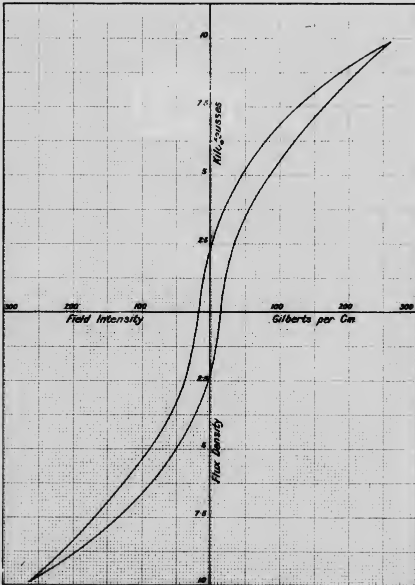
Fig. 9. Hysteresis Loop for Pure Cobalt - Sample H 217
