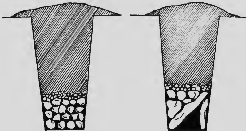
FIG. 83.— CROSS-SECTIONS OF STONE-DRAINS
