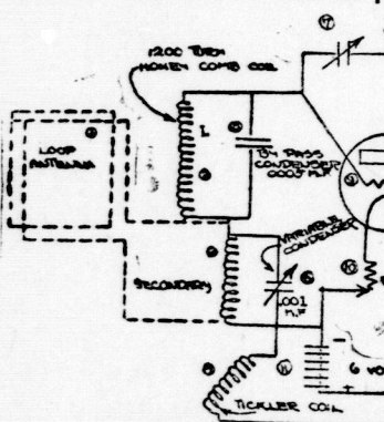
SUPER-REGENERATIVE RECEIVER CIRCUIT
