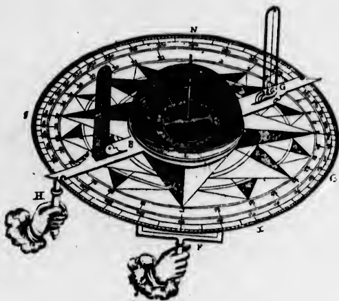
PRISMATIC COMPASS.
