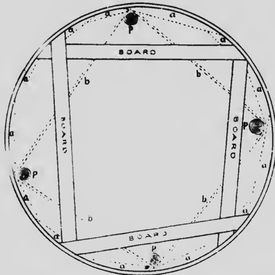
FIG. 4.—Plan of interior scaffolding, a, a, a , etc., boards cut \frac{1}{4} segments of 20 feet circle; b, b, b, b , braces nailed to p, p, p, p posts and extending to support circular platform made up of a, a, a , etc.
