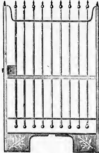
No. 7. Polished Brass Wicket. 18 in. wide, 24 in. high; each, $20.00. With lock and hinges.
