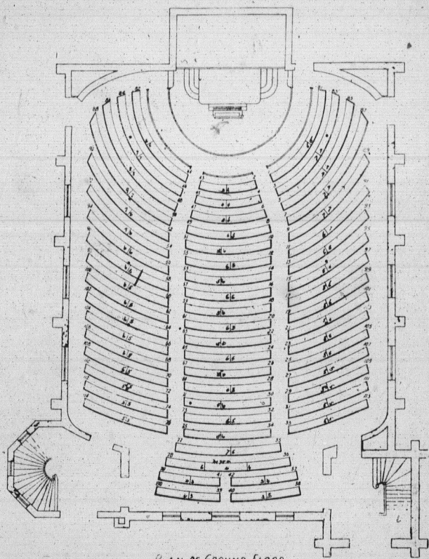
PLAN OF GROUND FLOOR
