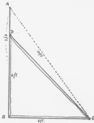
To make a right angle
