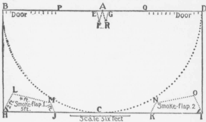
Pattern of 10-Foot Teepee.
