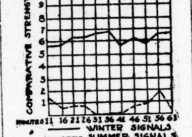
DIAGRAM SHOWING "SWINGING" OF WINTER AND SUMMER SIGNALS.
