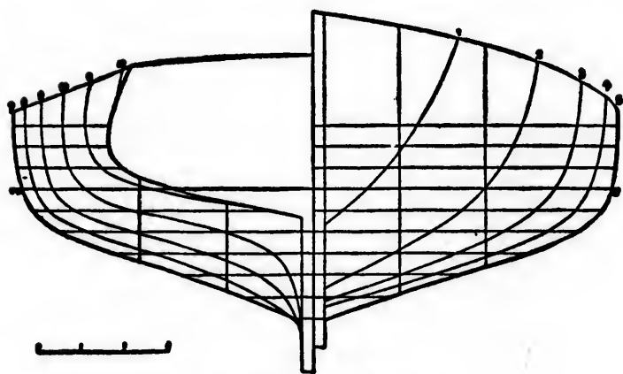
Body-plan of the Spray .
