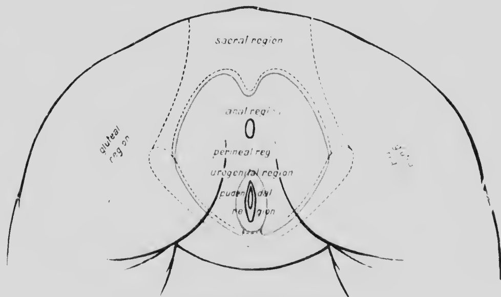
Fig. 235. Female perineum.
