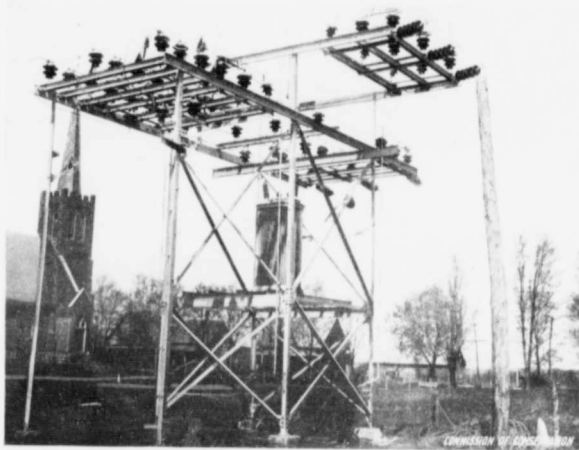
OUTDOOR SUBSTATION, SOUTHERN CANADA POWER CO.'S SYSTEM, QUE.
