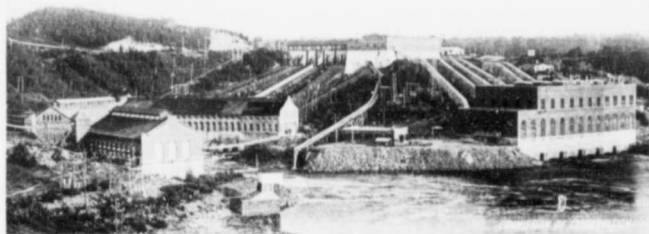
HYDRO-ELECTRIC PLANTS AT SHAWINIGAN FALLS, ST. MAURICE RIVER, ST. MAURICE CO. QUE. TOTAL CAPACITY, 185,000 H.P.
