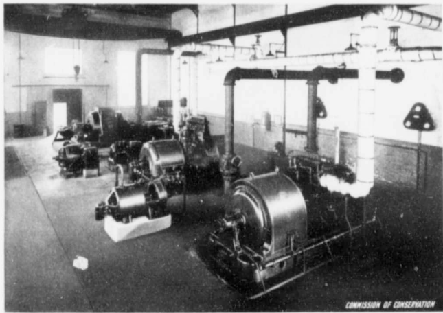
MUNICIPAL STEAM PLANT, MOOSE JAW, SASK.—STEAM TURBINE UNITS.
