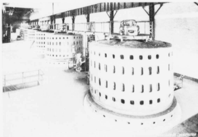
TORONTO POWER CO.—INTERIOR OF HYDRO-ELECTRIC PLANT, NIAGARA FALLS, ONT.
