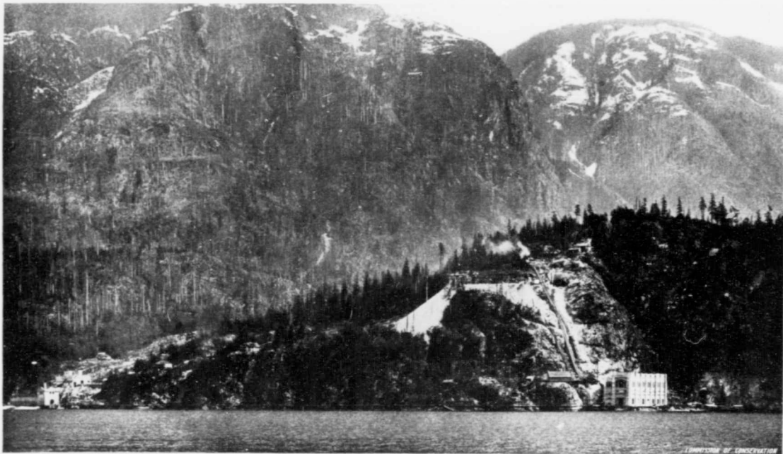
BRITISH COLUMBIA ELECTRIC RAILWAY CO.—COQUITLAM-BUNTZEN DEVELOPMENT, POWER PLANT ON NORTH ARM, BURRARD INLET, 16 MILES NORTHEAST OF VANCOUVER.—POWER HOUSE NO. 1 ON LEFT; POWER HOUSE NO. 2 ON RIGHT.
