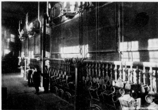
MUNICIPAL STEAM PLANT, MEDICINE HAT, ALTA.—BOILERS USING NATURAL GAS FUEL.
