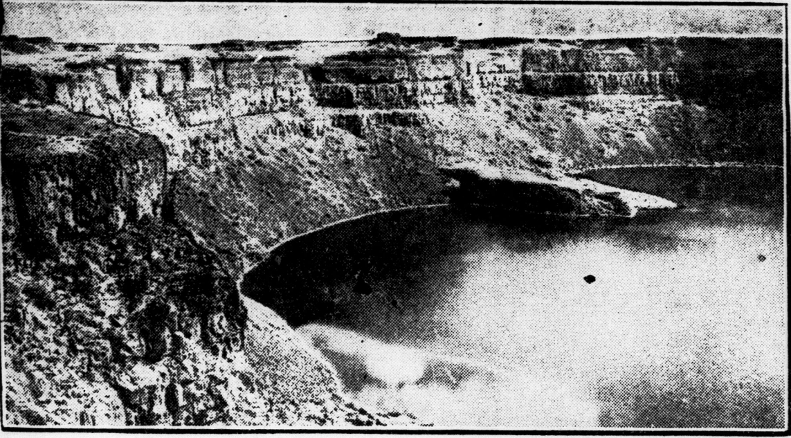
The dry falls at Grand Coulee, Wash., which geo logists believe at one time were similar to Niagara, the Columbia river once tumbling over the cliff s.
