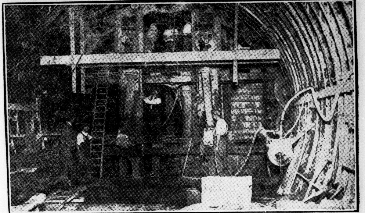
Flashlight photograph showing the construction under the Thames of the new railway tubes extension of Charing Cross, London.
