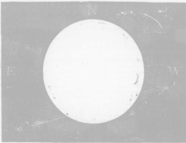
Diagram of the Transit of Venus across the Sun's Disc, December 6th, 1882.
