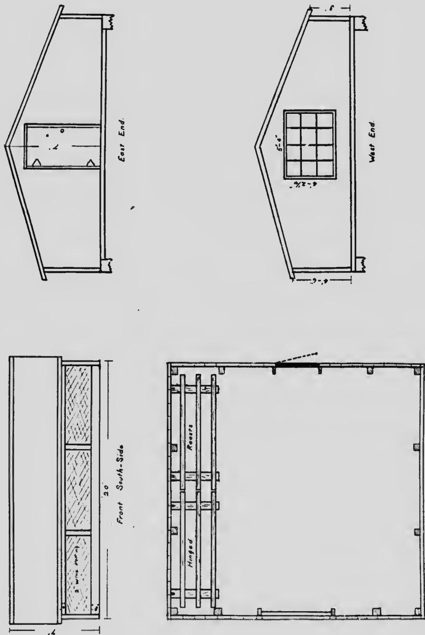
Fig. 26.—Open Front Poultry House.
