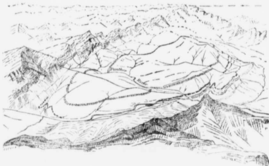
Figure 8. Sketch of Costigan coal-field.
