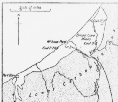
Figure 6. Broad Cove coal-field.
