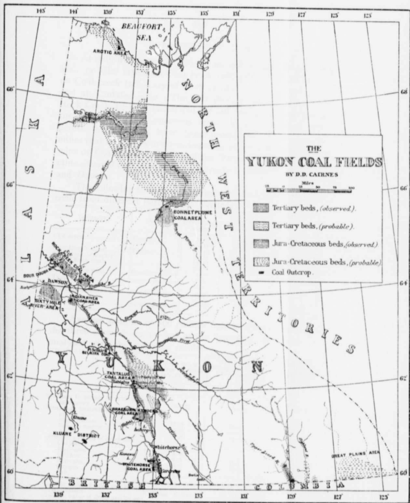
Figure 9. Yukon coal-fields.
