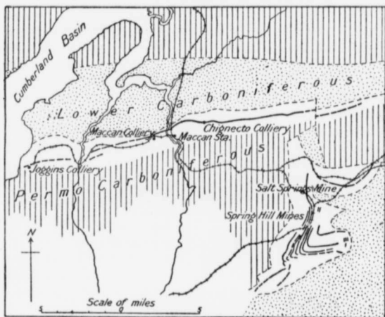
Figure 2. Coal-fields of Cumberland county.
