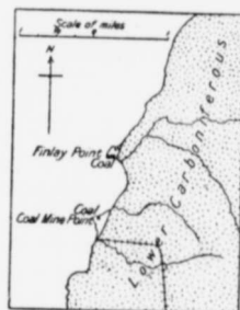
Figure 5. Mabou coal-field.
