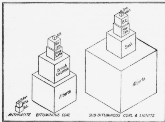
Figure 1. Diagram showing distribution of Canadian coal.
