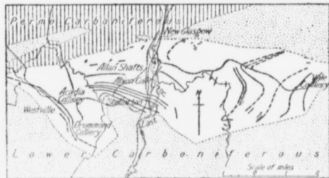
Figure 3. Pictou coal-field.
