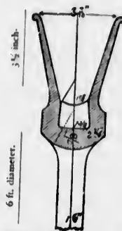
Section of Rim of 6 foot Wheel.
