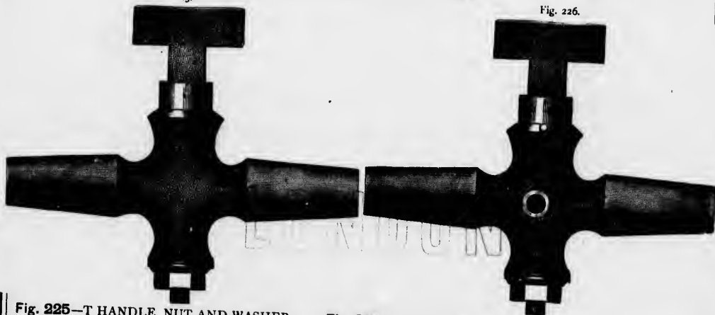
Fig. 226—T HANDLE, NUT AND WASHER, WITH WASTE
