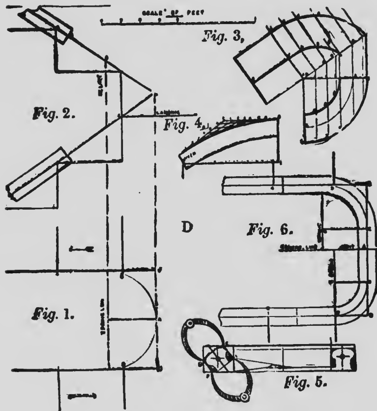
DIAGRAM D. HALF-SPACE RAILING
