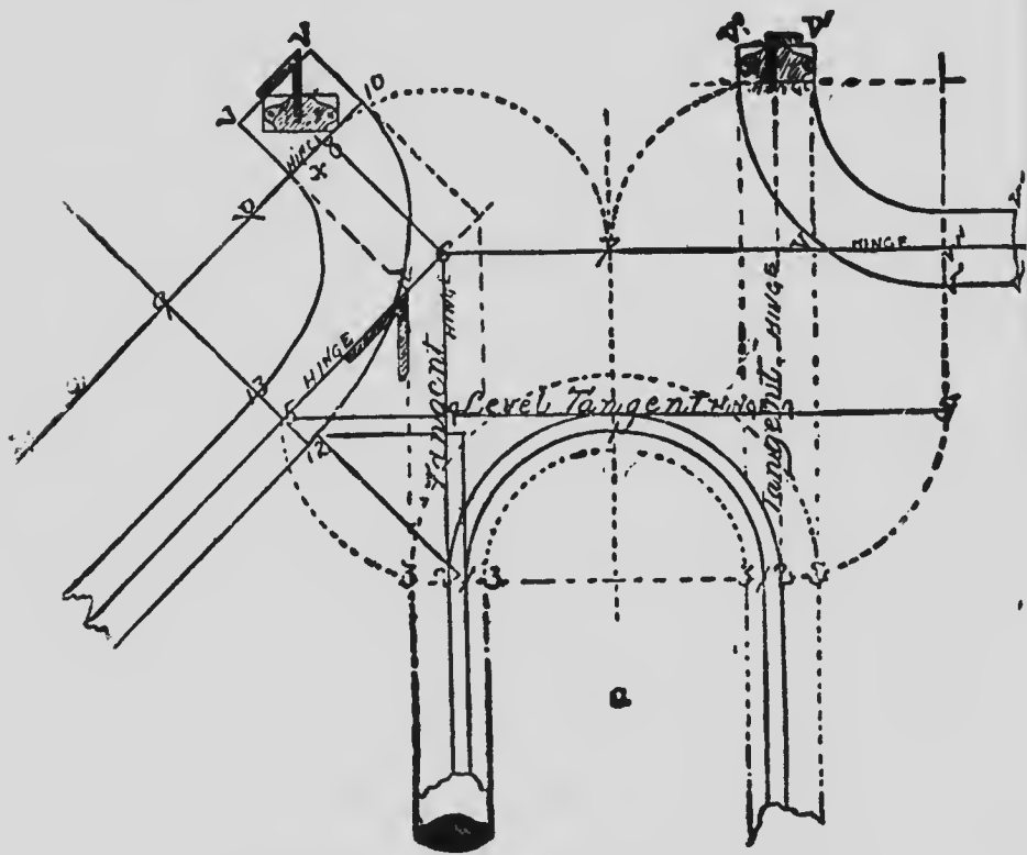
DIAGRAM C. A RAIL AROUND A CYLINDER
