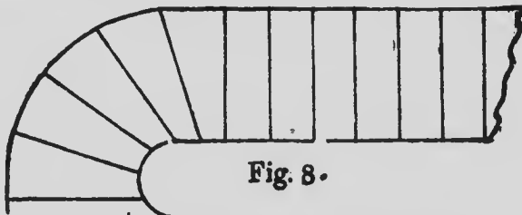
Fig. 8 shows the plan of a stair having five "dancing winders."
