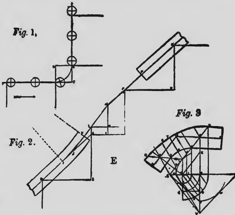
DIAGRAM E. QUARTER-SPACE RAILING
