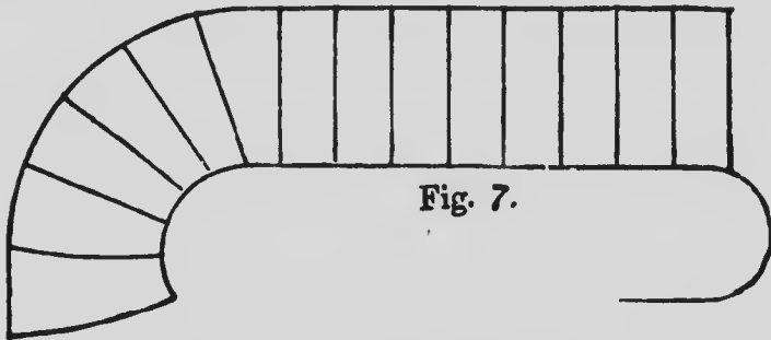
Fig. 7 is the plan of a stair similar to Fig. 6, but having seven winders.
