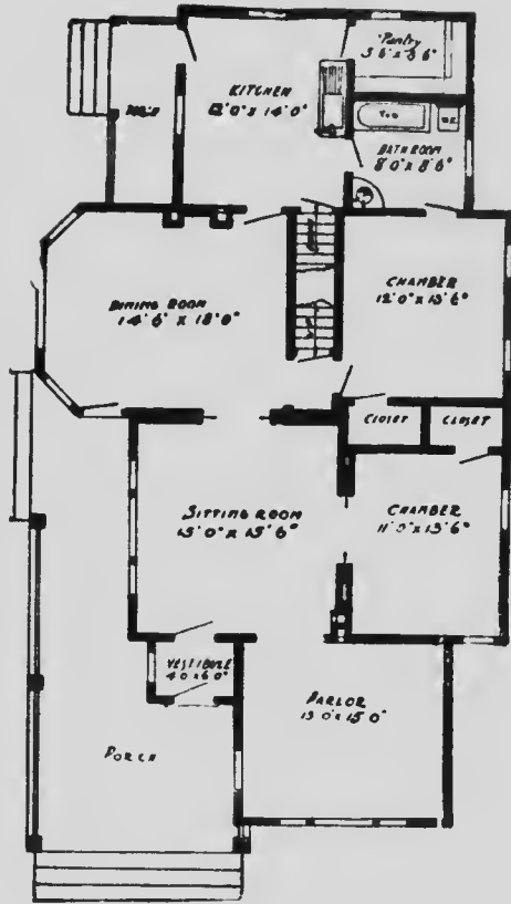
FLOOR PLAN
