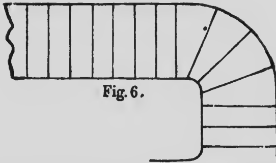
Fig. 6 shows a plan of a quarter-space stair with four winders.
