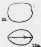
Matheria brevis . Fig. 25. Side view of the most perfect specimen collected, in outline, and showing the marginal contour of the right valve. Fig. 25 a. The same specimen, as seen from above, to show the amount of convexity of the closed valves. Both of these figures are of the natural size.
